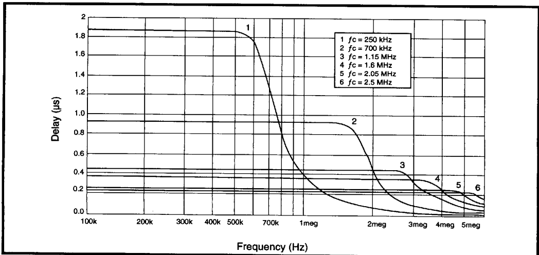
FIGURE 3: Typical Normal/Differentiated Output Group Delay Response
