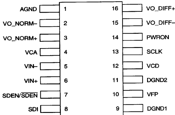
16-Lead SOL
